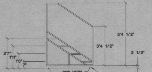
ROLLING STAIRS - SIDE VIEW
