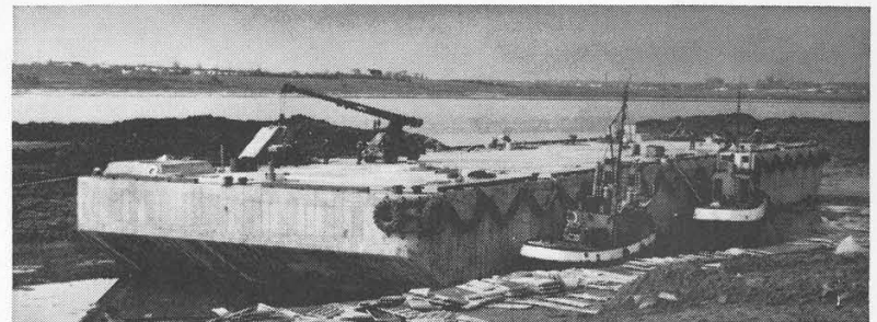
Dorchester Floating Dock, Chartersville, N.B.
