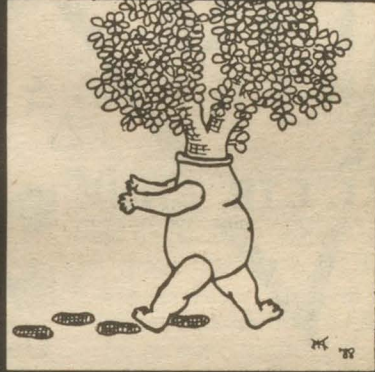
Backtracking
