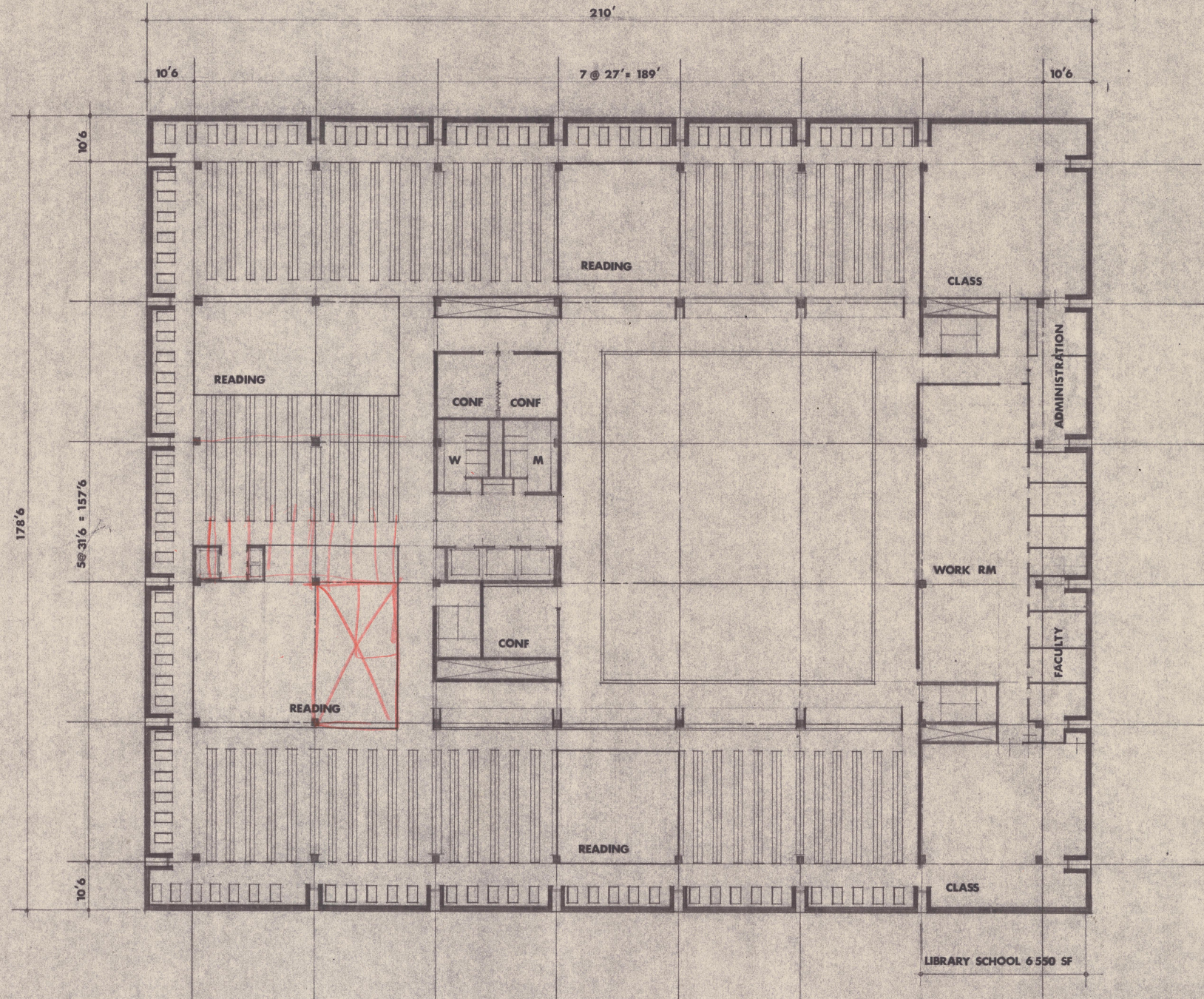
3 R D F L O O R 1/16" = 1' - 0" 0' 20' 40'
